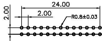
DIP P.C.Board Layout (TOLERANCE=±0.05)
